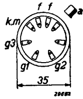
Fig. 2 Arrangement of electrodes and contacts.
