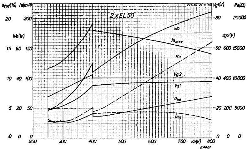
Fig. 11 Maximum anode current I_{ama} , standing current I_{a0} , screen voltage V_{g2} , grid bias V_{g1} , output power W_o , total distortion d_{tot} and optimum output impedance R_a as a function of available anode voltage V_a of two EL 50 valves in a push-pull circuit with fixed grid bias.
