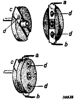
Fig. 2 Construction of a low-value differential condenser. Top; Left and right half-sections of the condenser. (a) stationary electrode; (b) second stationary electrode; (c) rotating plate, adjustable with respect to electrodes (a) and (b); (d) eyelets, by means of which the electrodes (a), (b) and (c) are attached to the bakelised paper discs. Bottom; The assembled condenser.
