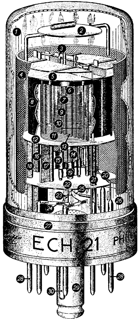
Fig. 3 Construction of the Miniwatt all-glass Triode-Heptode ECH 21
