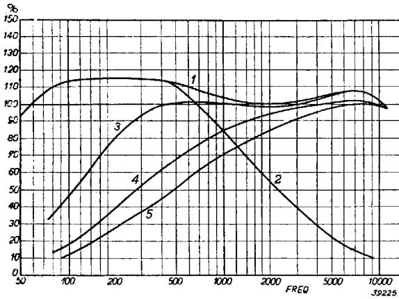
Fig. 2 Frequency characteristic of the amplifier.
