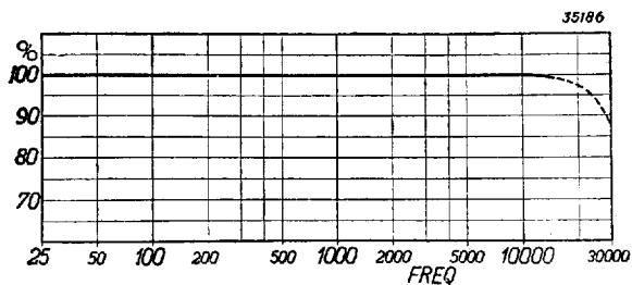
Frequency characteristic of the instrument.
