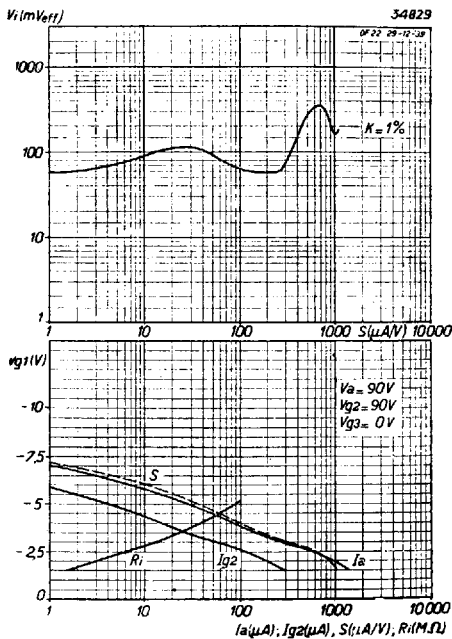
Fig. 8 Upper diagram; Effective value of alternating grid voltage as a function of mutual conductance, with 1 % cross modulation, at V_a = V_{g2} = 90 V.
