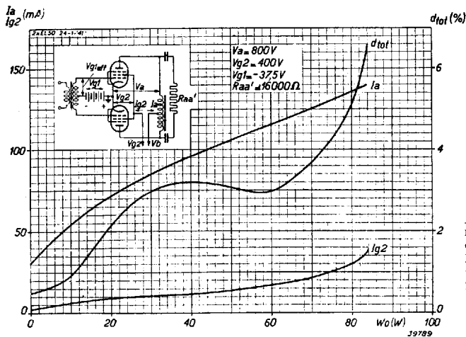
Fig. 9 Anode current I_a , screen current I_{g2} and total distortion d_{tot} as function of the output power W_o of two push-pull EL 50 valves, with fixed grid bias, at V_a = 800 V, V_{g2} = 400 V and V_{g1} = -37.5 V; R_{aa}' = 16,000 Ohms.
