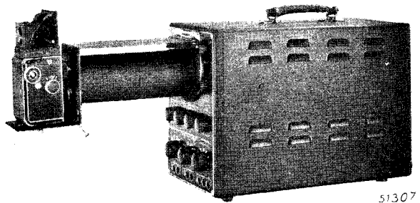
Fig. 3 Stand, GM 4193, mounted on the Cathode Ray Oscilloscope GM 3156 and supporting a "Rolleicord" camera.
