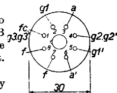
Fig. 2 Arrangement and sequence of contacts.
