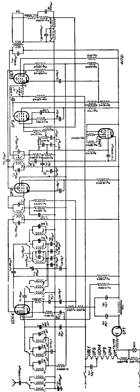
Circuit diagram of 4-valve superheterodyne receiver for 230 V AC/DC mains operation. (Published without any guarantees in respect of patent rights.)
