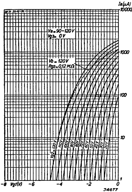
Fig. 4 Anode current as a function of grid bias at V_a = 90 - 120 \text{ V} , with V_{g2} as parameter. The broken line represents the conditions for the controlled valve, with the screen fed from the 120 V source through a resistance of 0.12 M Ohm.
