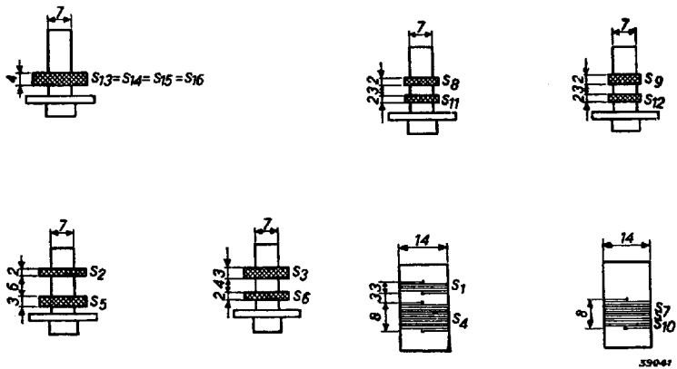
Fig. 2 Sketches of coils used in this 3-valve receiver.
